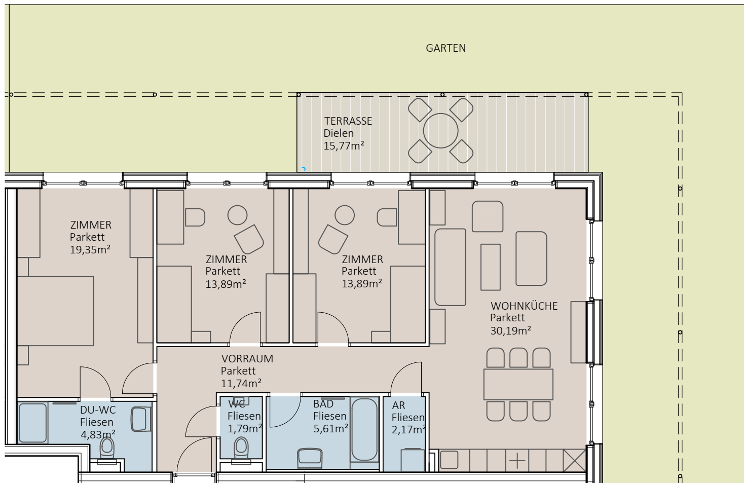
TOP A_06 103,46m 2
